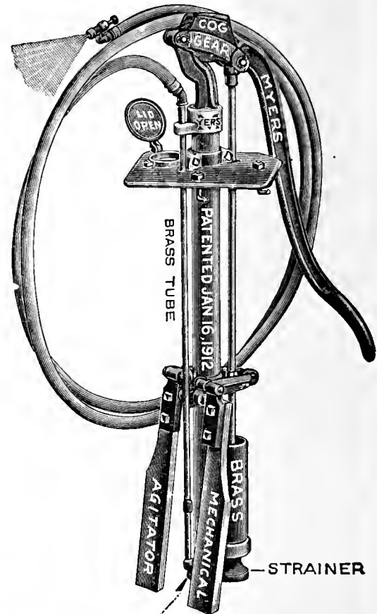
Cog Gear, Cylinder, Valves, Valve Seats and Discharge All Brass.
